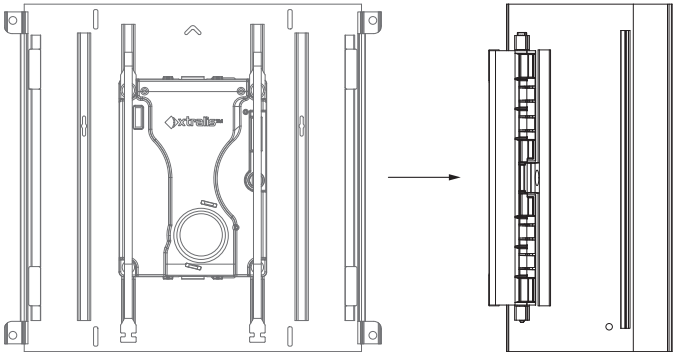
Figure 4-10: Detaching door
