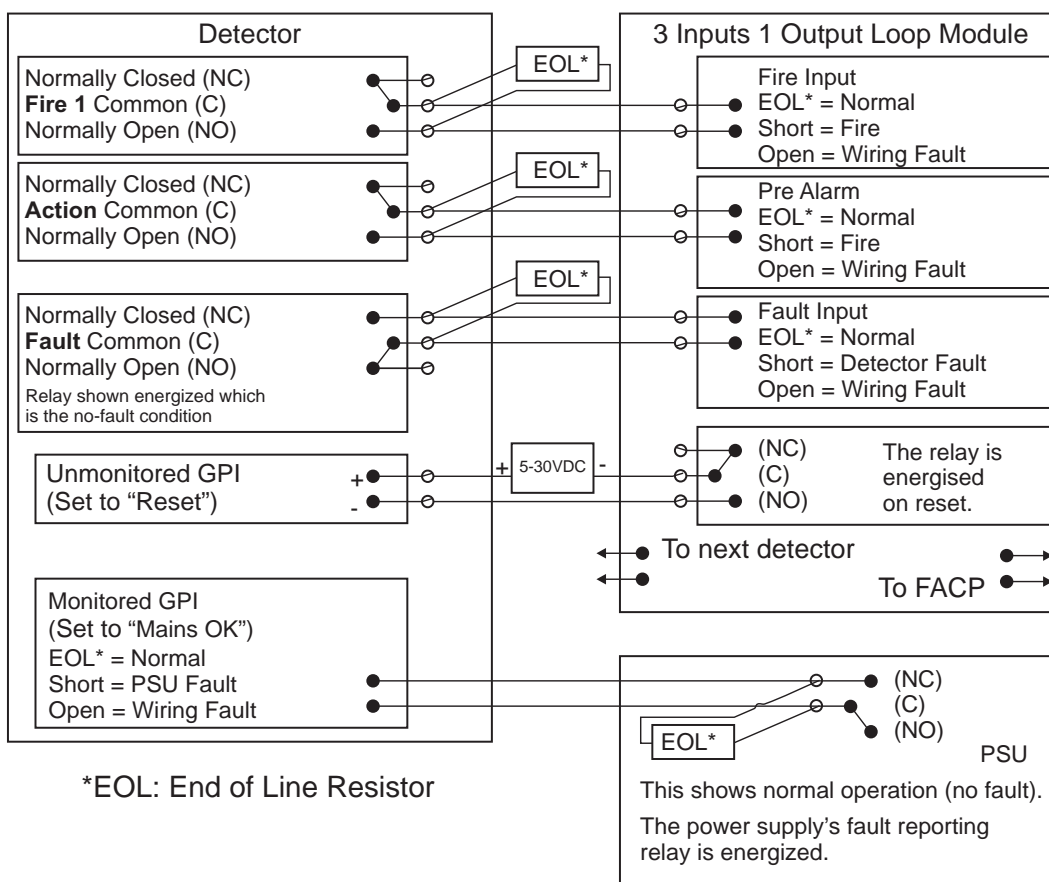
Figure 4-38: Input/Output Loop Module with EOL
