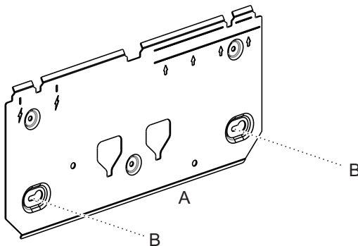
Figure 4-18: Mark keyholes
