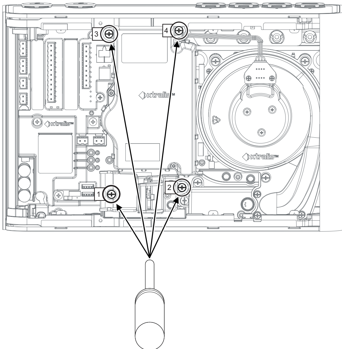
Figure 7-13: Undo Chamber retaining screws
