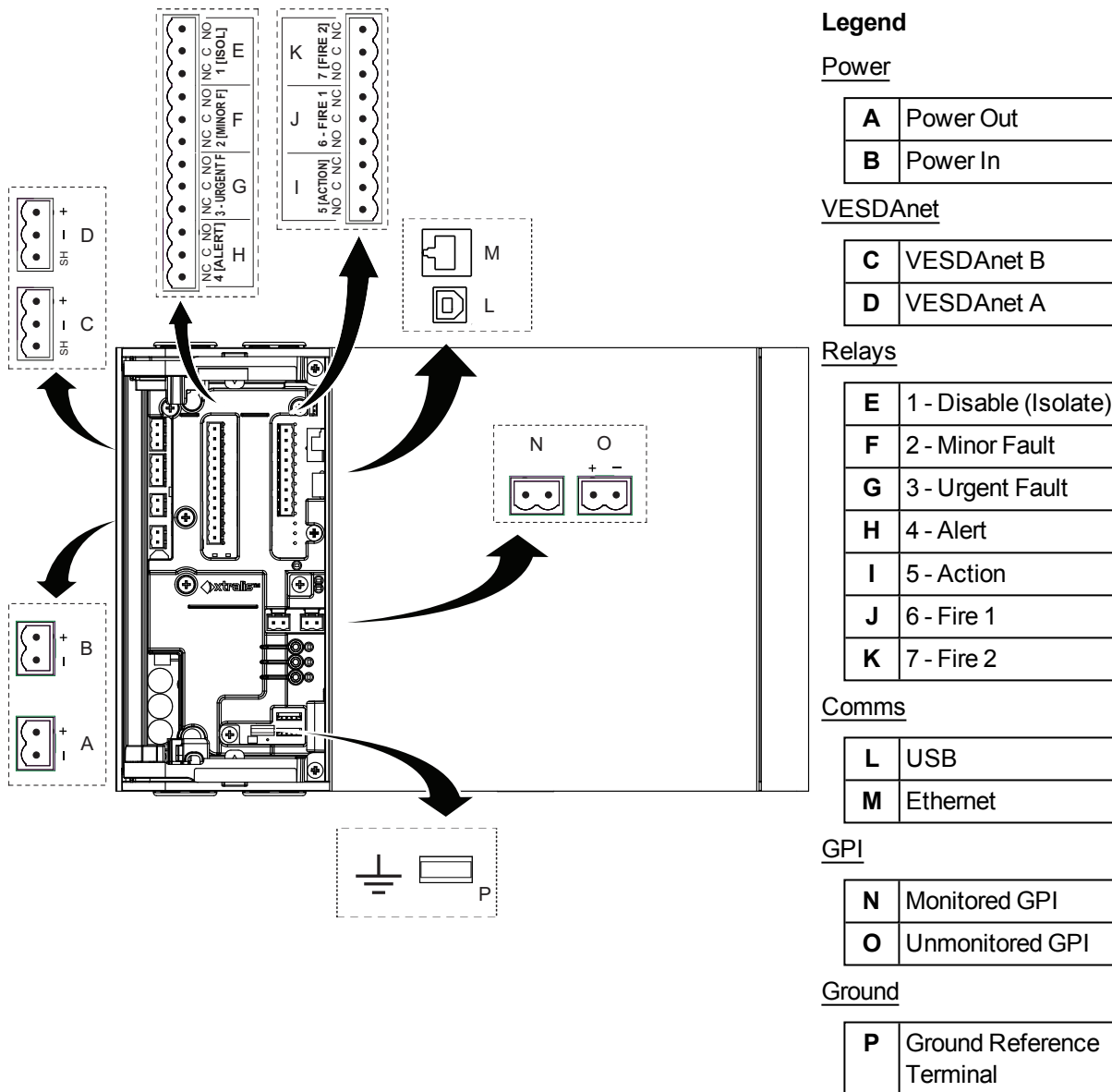
Figure 4-33: Socket Locations
